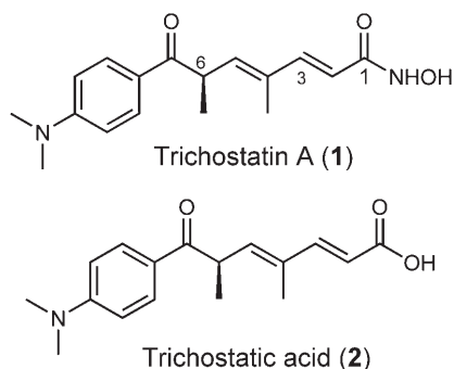
Figure 1. (+)-Trichostatin A ( 1 ) and trichostatic acid ( 2 ).
