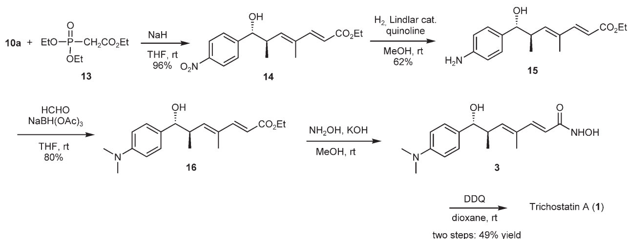
Scheme 4. Synthesis of trichostatin A ( 1 ).
