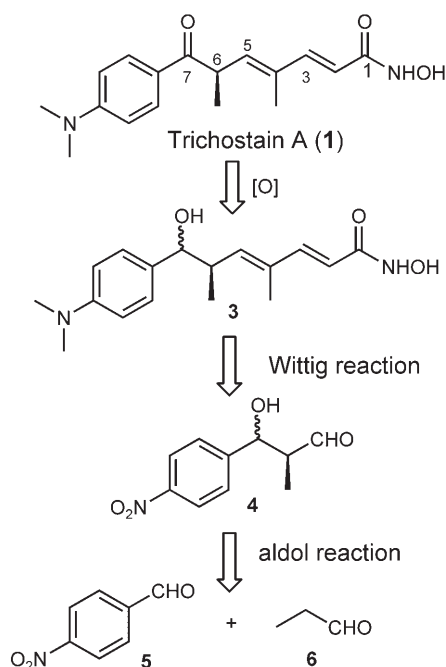
Scheme 1. Retrosynthetic analysis of trichostatin A (1).
