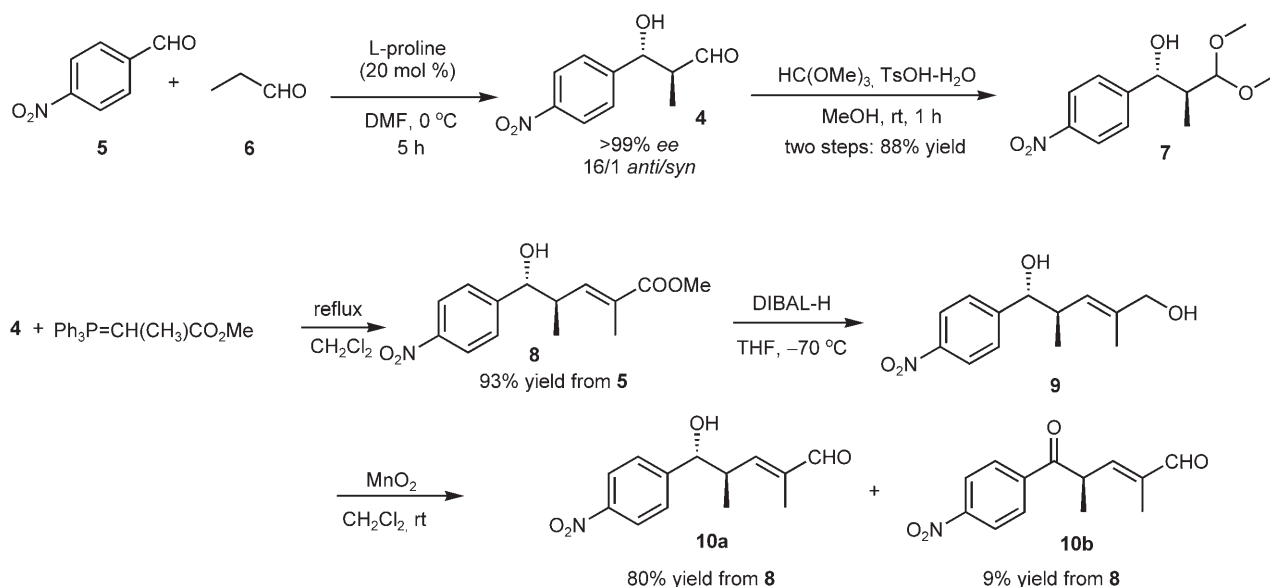
Scheme 2. Synthesis of intermediate 10a .
