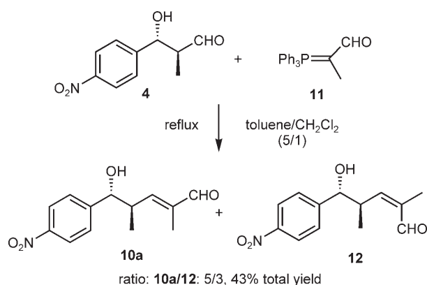
Scheme 3. An alternative approach to synthesis of 10a .
